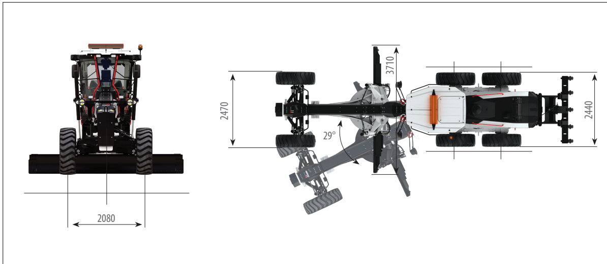
Dimensions (I)
