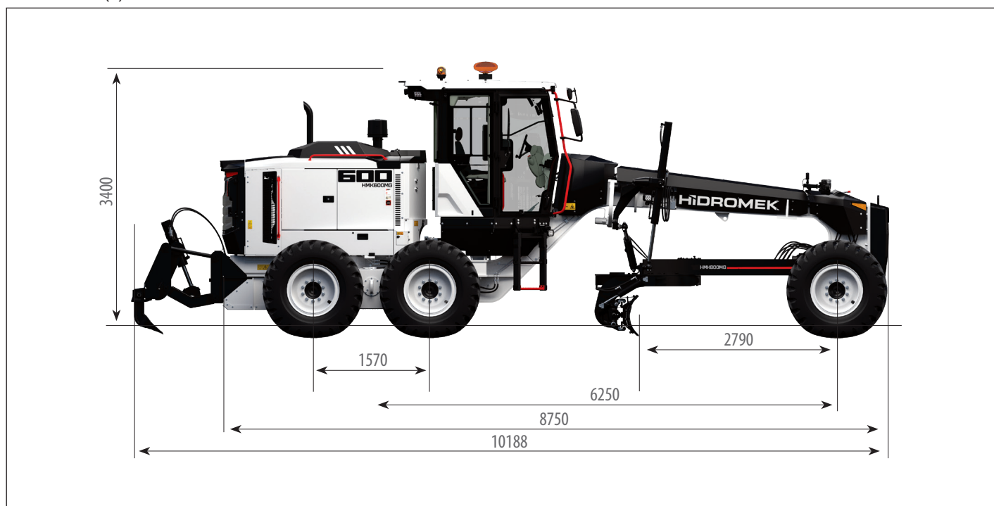
Dimensions (II)
